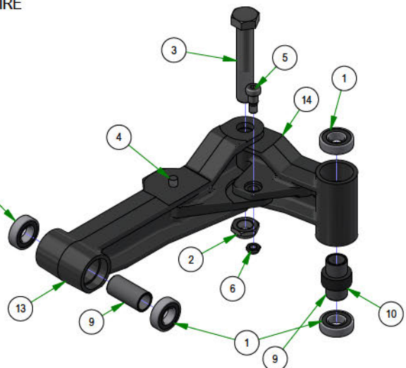
250-0033-03 LH FRONT SUSPENSION ARM
