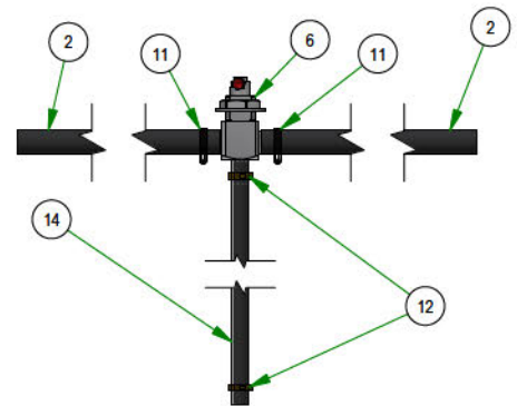
051-2019-33 FUEL LINE ASSEMBLY KOHLER VANGUARD FX1000 EFI
