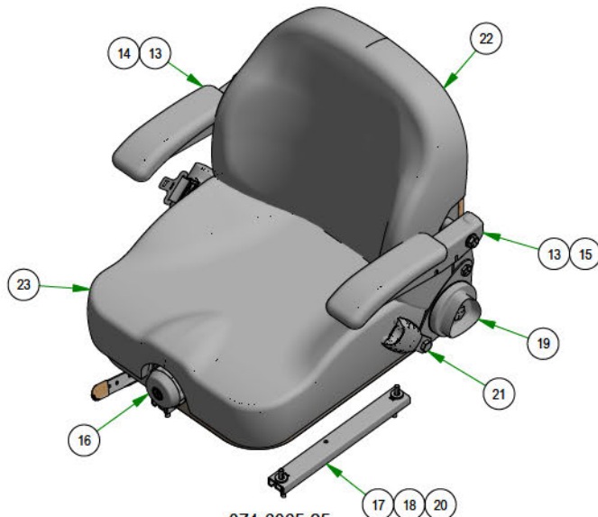
071-6065-25 SEAT ASSEMBLY
