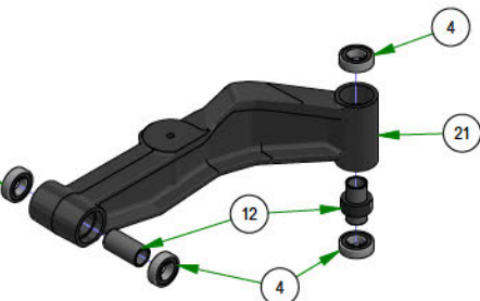
250-0032-54 LH FRONT SUSPENSION ARM 54" DECK
